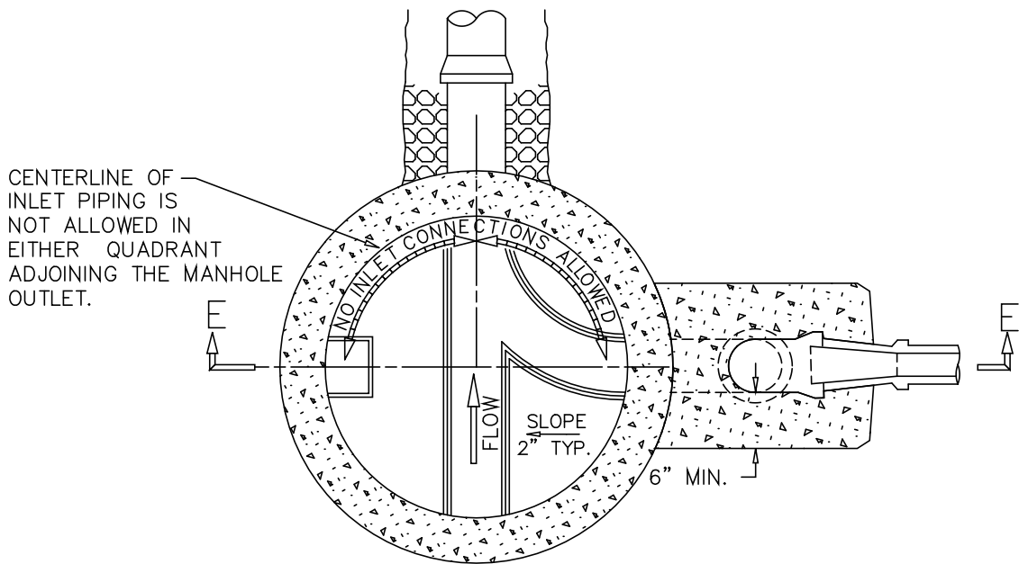
SECTIONAL PLAN
