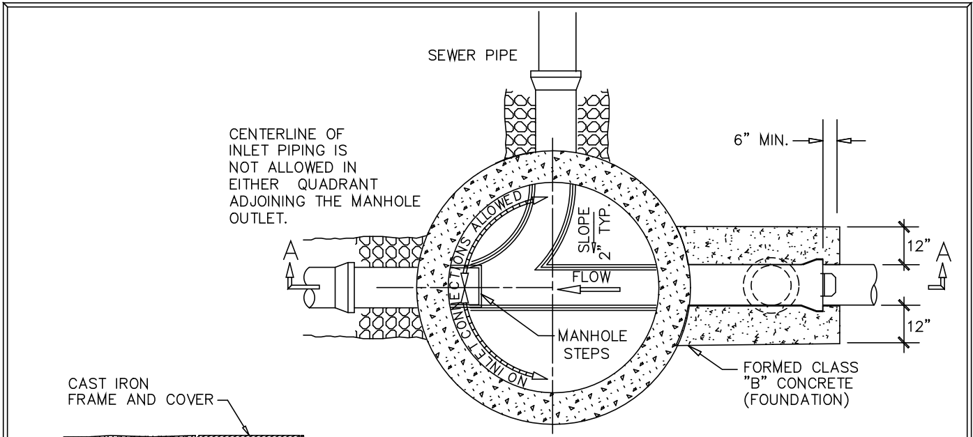
PLAN SECTION
